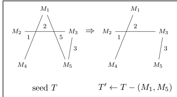
Figure 4: Lines 4 and 5 of Algorithm 2.
